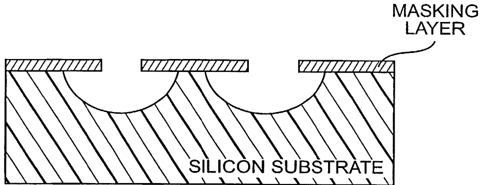
CROSS-SECTIONAL VIEW OF THE ETCH PROFILE OF ISOTROPIC ETCHING FOR VARYING TIMES.
